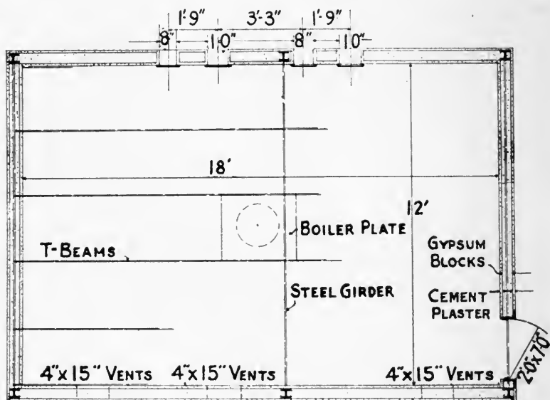
FIG. 5. Reflected ceiling plan of projection room.
